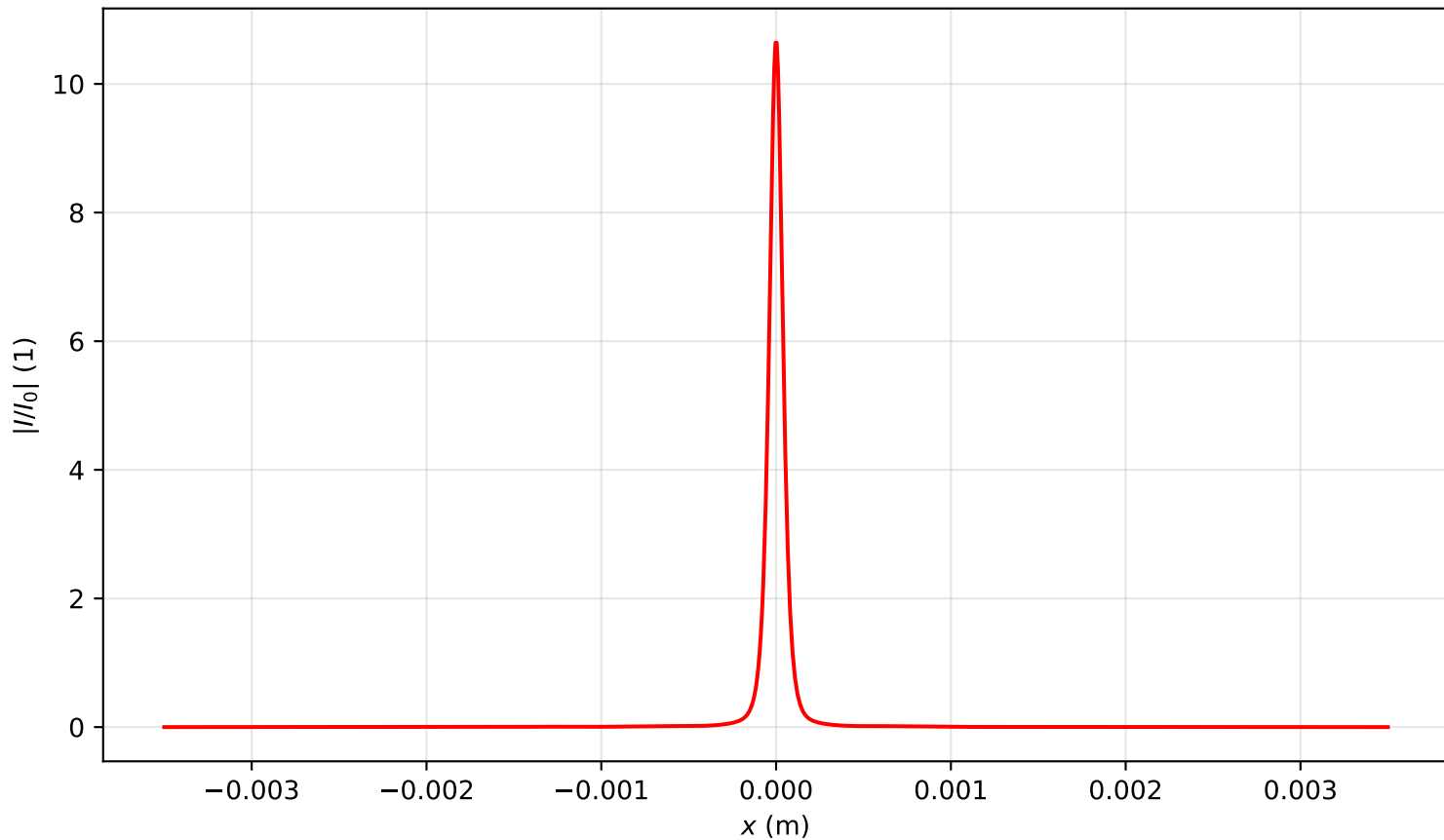
Intensity profile I(x, y = 0, z = 3.503)/I_0 , P_{in}=4.0P_{cr} , artificial time
